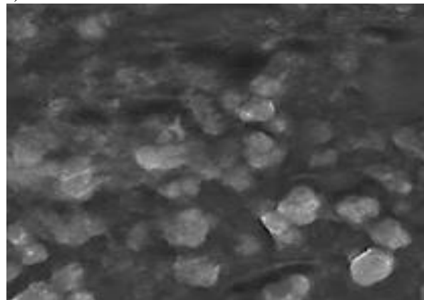
Fig. 3: SEM image of prepared silver nanoparticles
