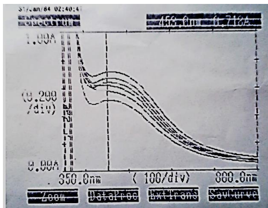
Fig. 2: The absorbance spectrum of silver nanoparticles showing maximum absorbance at 453nm
