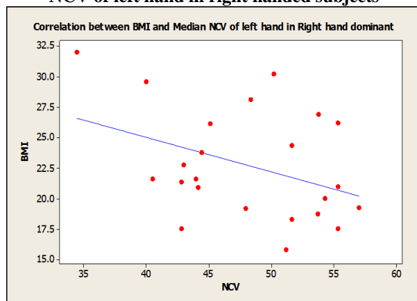
Graph 2: Correlation between BMI and Median NCV of left hand in right handed subjects
