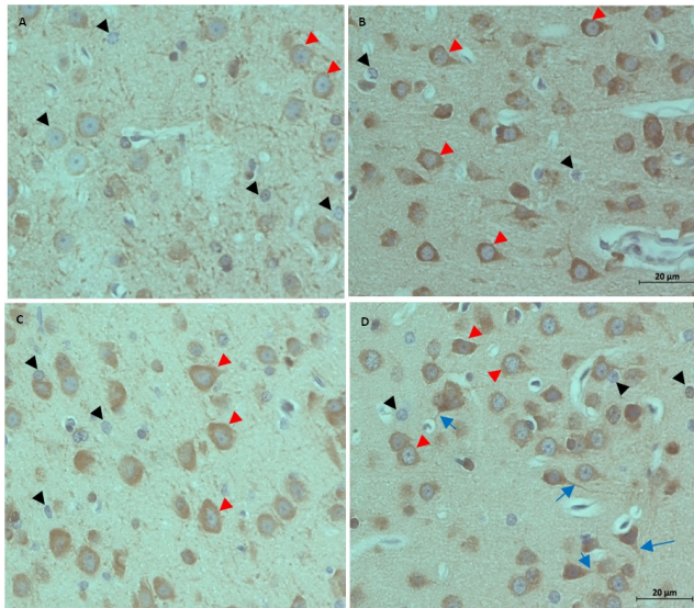
Fig. 3: Prefrontal cortex of the control group showing abundance of pyramidal neurons (black arrow heads) that do not take up the DCX stain (arrowheads), B: Shows group 1 (500 mg/kg) with increased DCX+ Pyramidal cells with brown staining of the cytoplasm within the cell body (red arrowheads) and less DCX-negative neurons (black arrowheads). C: Demonstrates prefrontal cortex of the experimental group 3 (1000mg/kg) showing a reduction in number of the DCX- Pyramidal cells (black arrow heads) in comparison to the control group, and lower density of DCX+pyramidal neuronal cells (red arrowheads) when compared to experimental group 1. In the 3 rd group ( D ), note the reduced density of DCX+ cells (red arrow heads) as compared to the other experimental groups. The processes of the neuron can also be noted on some neurons (blue arrows) (Nissl stain with DCX counterstain). Magnification = x400
