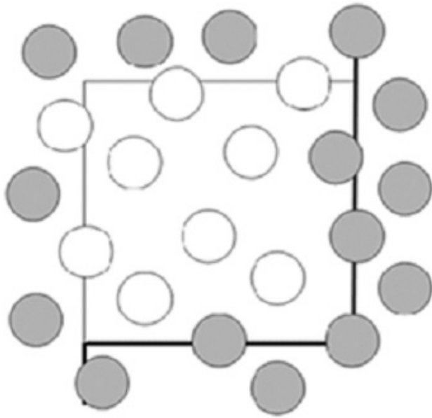
Fig. 1: An illustration of the cell counting method. The bold lines represent the exclusion zone while the lighter lines represent the inclusion zone. All cells within the area bounded and touching the inclusion zone were counted
