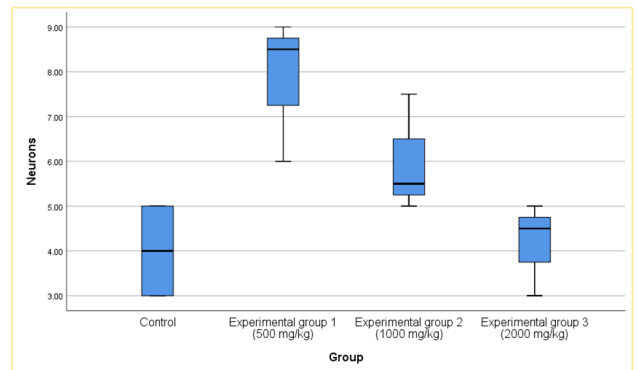
Graph 1: Box plots of the DCX-positive pyramidal neuronal densities in each study group
