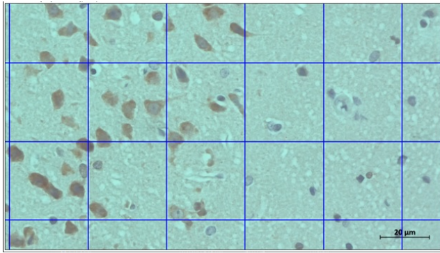
Fig. 2: Figure displaying the grids used to determine the immature neuronal densities
